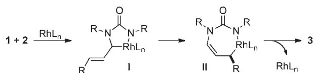
Scheme 1. Mechanistic Proposal
